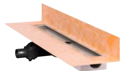
Schlüter-KERDI collar, upright for wall installation
