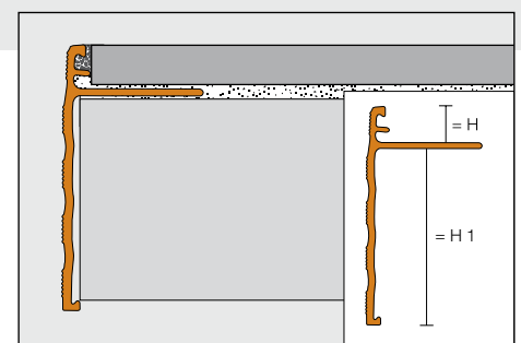
Schlüter®-SCHIENE-STEP-AE
