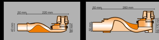
Schlüter®-KERDI-LINE-VARIO-H 40
