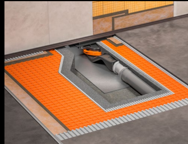
Schlüter®-KERDI-LINE-VARIO-H 40
