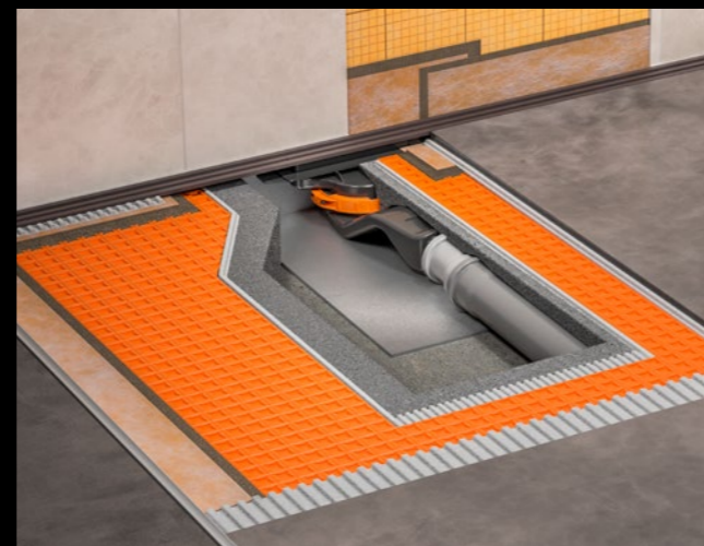
Schlüter®-KERDI-LINE-VARIO-H 40
