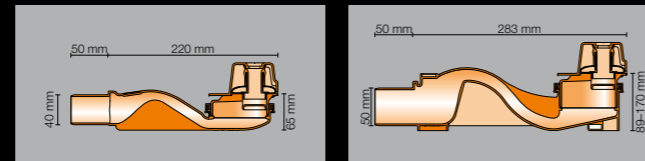
Schlüter®-KERDI-LINE-VARIO-H 40
