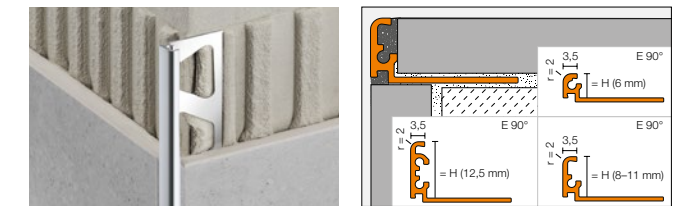
Schlüter®-JOLLY
