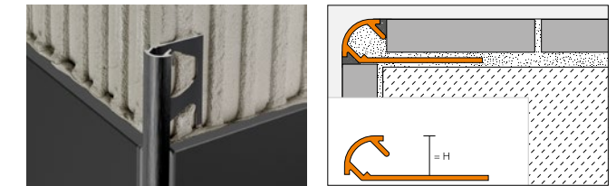
Schlüter®-RONDEC
