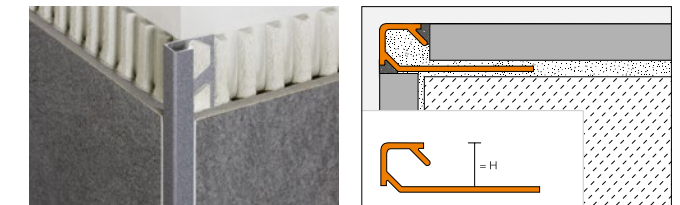
Schlüter®-QUADEC
