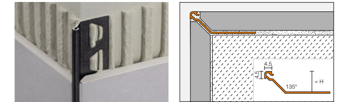
Schlüter®-FINEC-SQ
