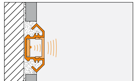
Wall mounting
