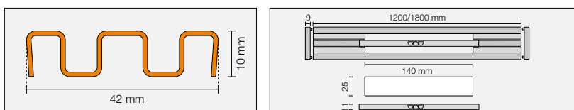
Schlüter®-KERDI-LINE-VARIO-WAVE-42 EB
