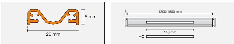
Schlüter®-KERDI-LINE-VARIO-COVE 26 A
