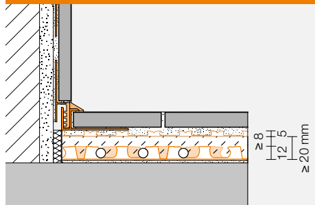
Schlüter®-BEKOTEC-THERM EN 12 FK
