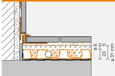
Schlüter®-BEKOTEC-THERM EN 23 F
