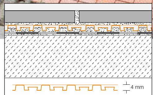
Schlüter®-DITRA-DRAIN 4
